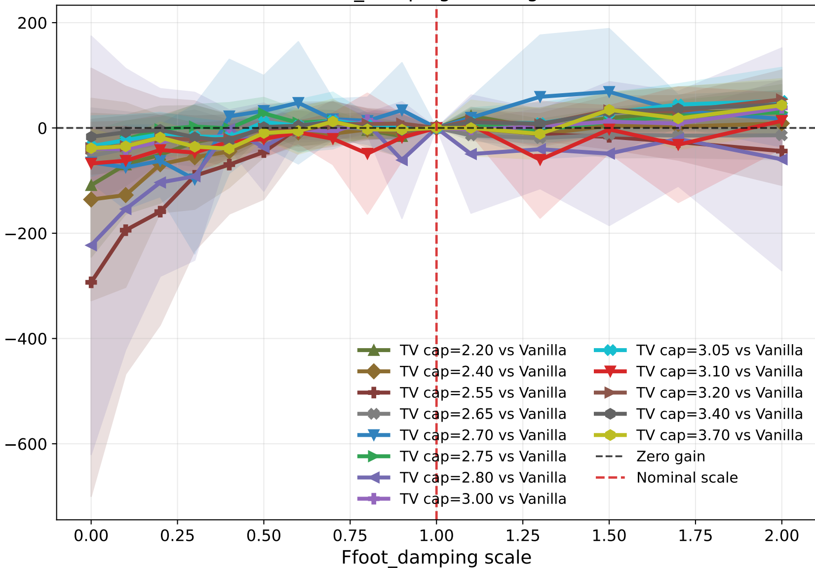
Ffoot_damping robust gain
